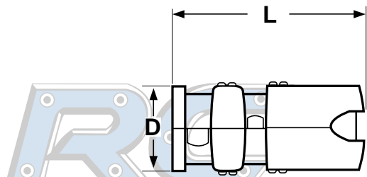
SINGLE EXPANSION
