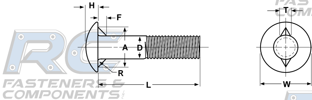
CARRIAGE BOLTS, FIN NECK
