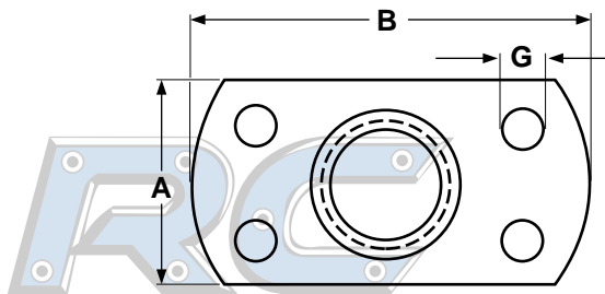
TAB WELD NUTS - CENTER HOLE DESIGN WITH MULTIPLE PROJECTIONS
